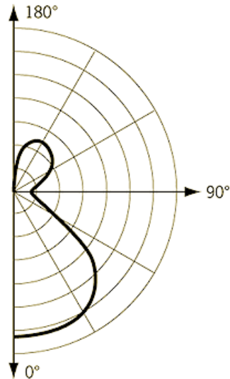
Goniometric diagram of a web distribution
