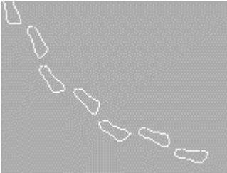
Bend=0.5
