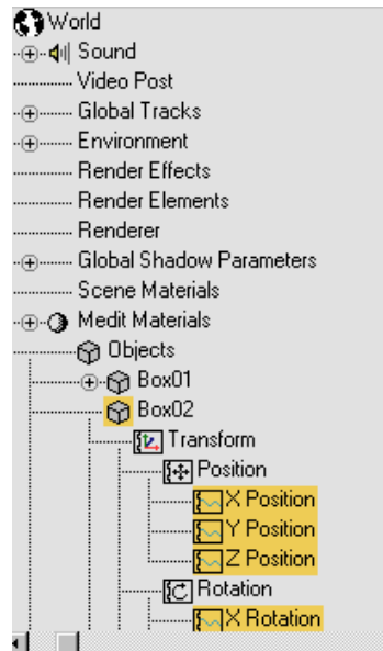
Controller window
