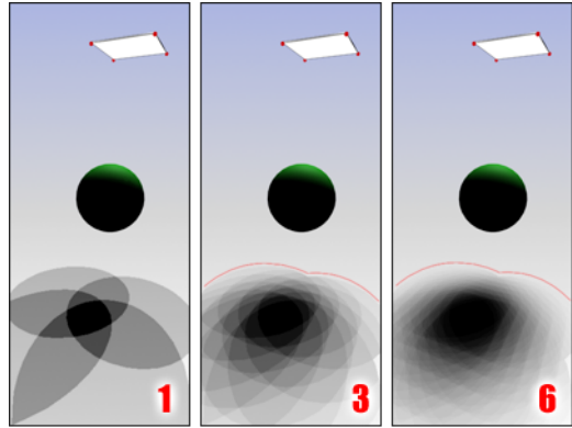
Increasing the Shadow Quality value produces a more accurate penumbra (soft area) within the contour defined by the Shadow Integrity value.
