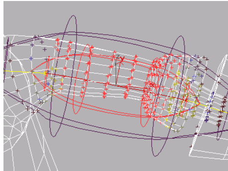
Envelopes
