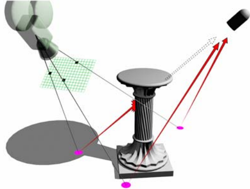
Ray-traced shadows
