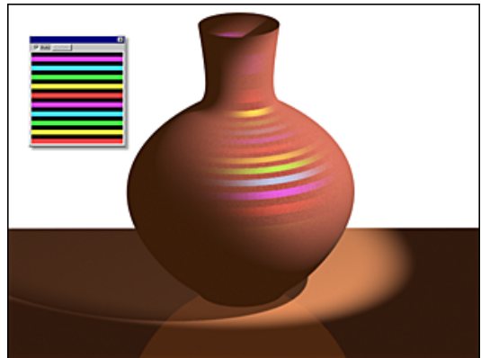
Mapping the specular highlight
